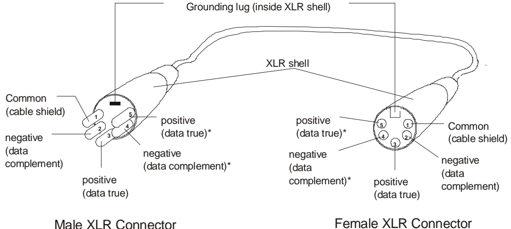
Male XLR Connector
