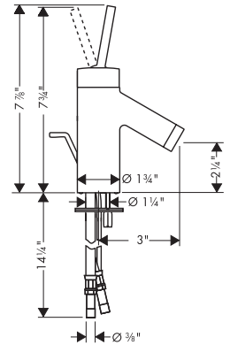
Starck single lever bidet mixer 10201XX1
