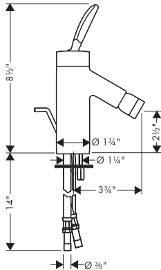
Starck single lever bidet mixer 10200XX1
