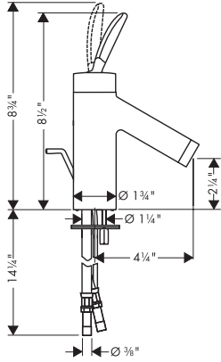
Starck single lever basin mixer 10015XX1
