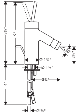
Starck single lever bidet mixer 10201XX1
