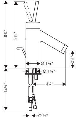
Starck single lever basin mixer 10016XX1
