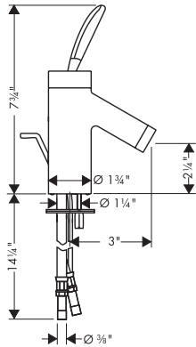
Starck single lever bidet mixer 10200XX1
