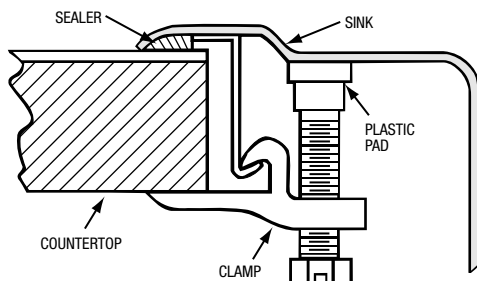
"J" Channel Type Installation Profile for Copper and Brass Sinks
