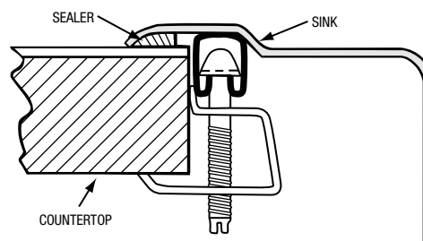
"U" Channel Type Installation Profile for Stainless Steel Sinks
