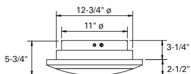
MODIFIED INTEGRAL EMERGENCY BATTERY (MEM)
