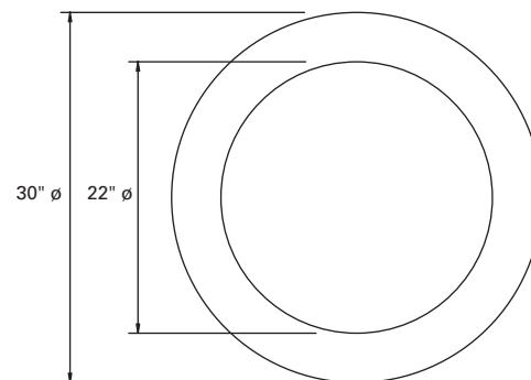
230 - 30" \varnothing STANDARD
