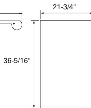
36" Vertical - Mirror Only
