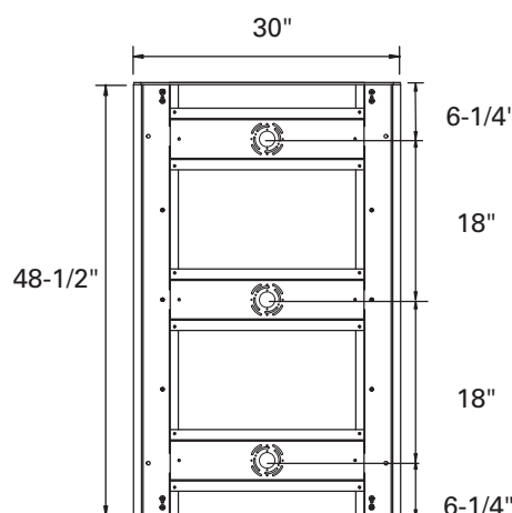
48" Vertical J-Box Mounting Location
