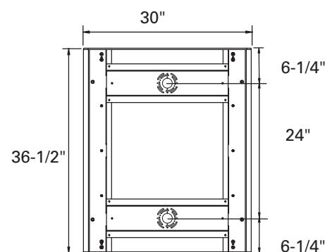
36" Vertical J-Box Mounting Location
