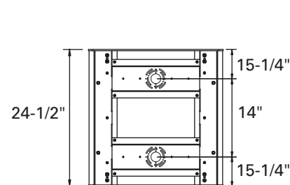
24" Vertical J-Box Mounting Location
