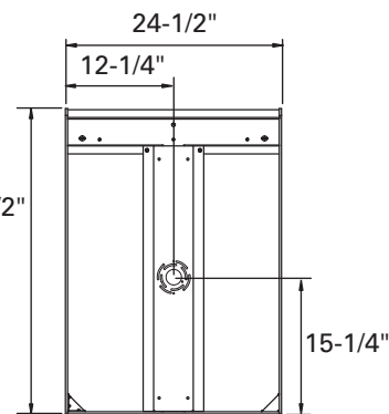
34" Horizontal J-Box Mounting Location
