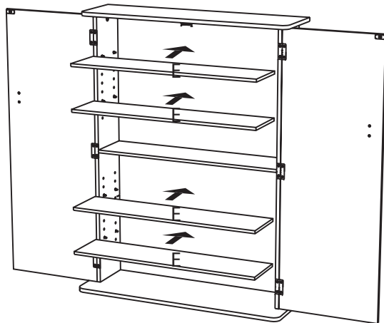
15- Place shelves (E) on top of pins (V)
