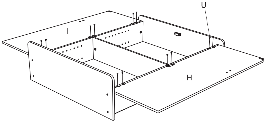
13 - Attach doors (H) & (I) to unit with screws (U).
