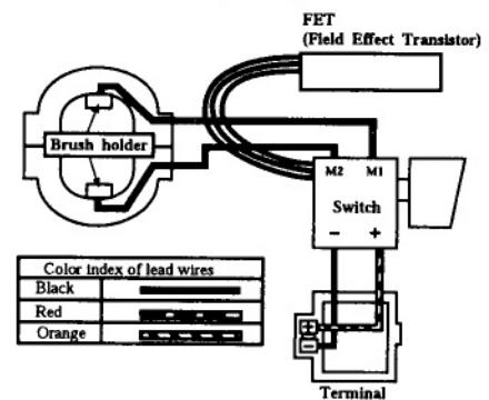
Wiring Diagram
