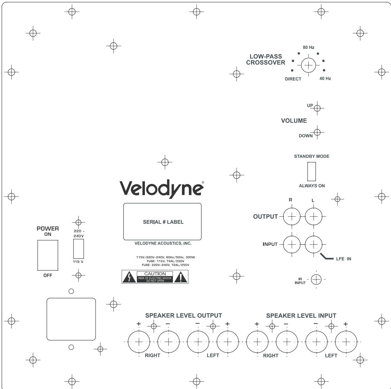
Figure 3. CHT-15Q Rear Panel Connections
