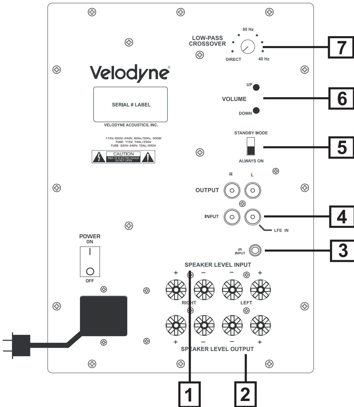
Figure 2. CHT-8Q, CHT-10Q, and CHT-12Q Rear Panel Connections
