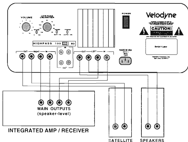
Figure 2: Installation using speaker-level (from amplifier) inputs
