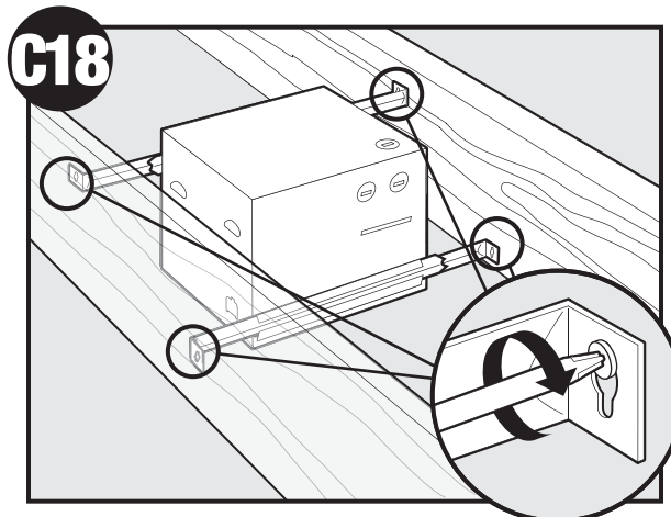
Tighten screws.
