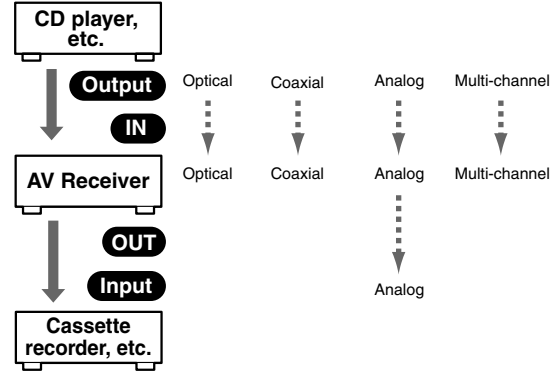
Audio Input/Output Diagram for Recording
