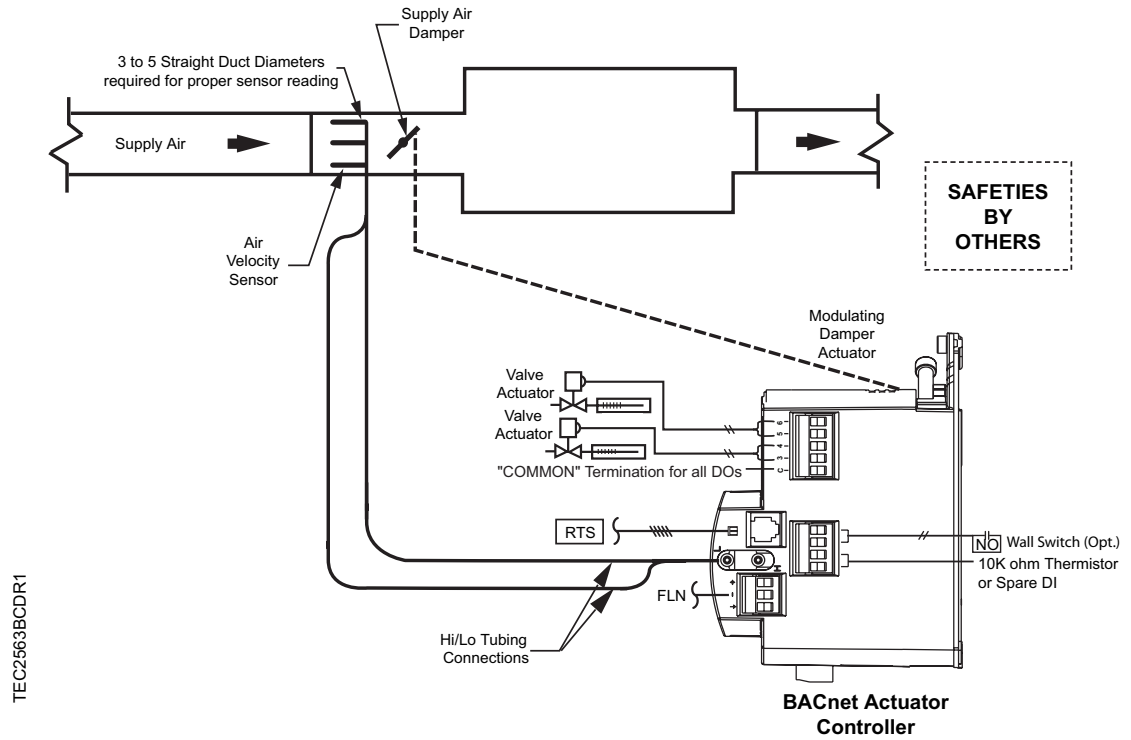
Figure 10. Application 2563 Control Drawing (Two Valve Actuators).
