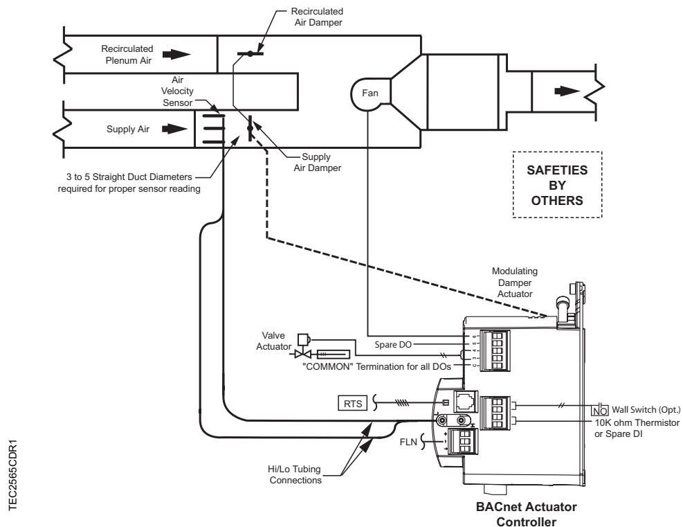
Figure 12. Application 2565 Control Drawing.
