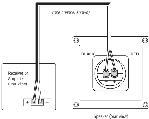
Figure 5. Wiring diagram shows polarity connections for one channel of a stereo or home theater system.
