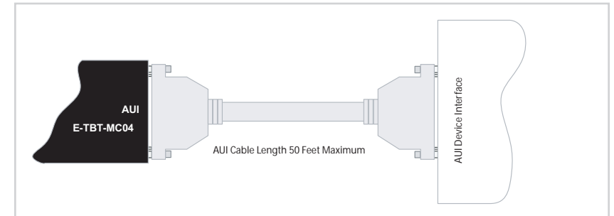
Figure 7: E-TBT-MC04 Connected to an AUI Device Port
