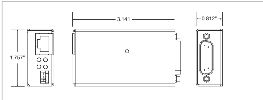
Figure 3: E-TBT-MC04 Dimensions
