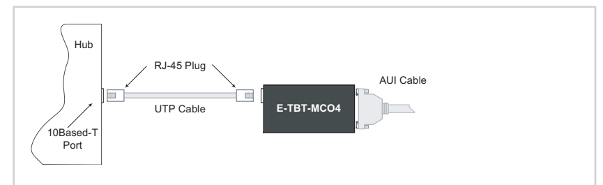
Figure 8: E-TBT-MC04 Connected to a RJ-45 Device Jack
