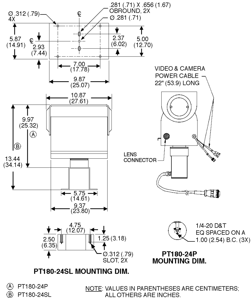
Figure 4. Mounting Dimensions
