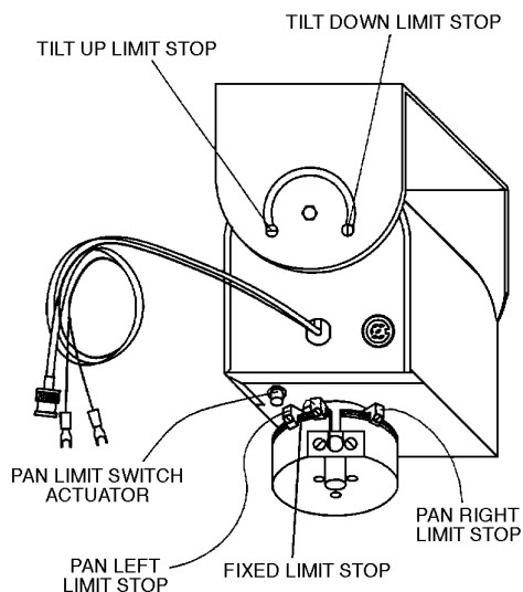
Figure 3. Limit Stops
