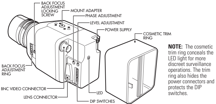
Figure 1. Camera Layout
