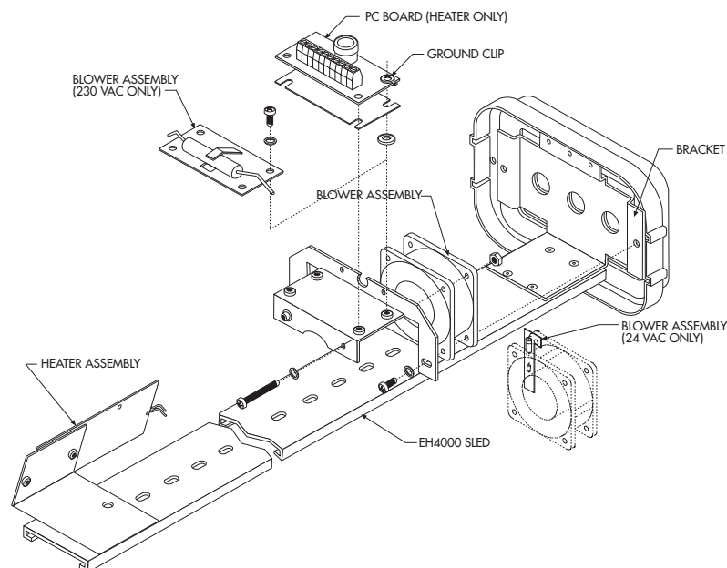
Figure 1. Blower/Heater Kit Installation
