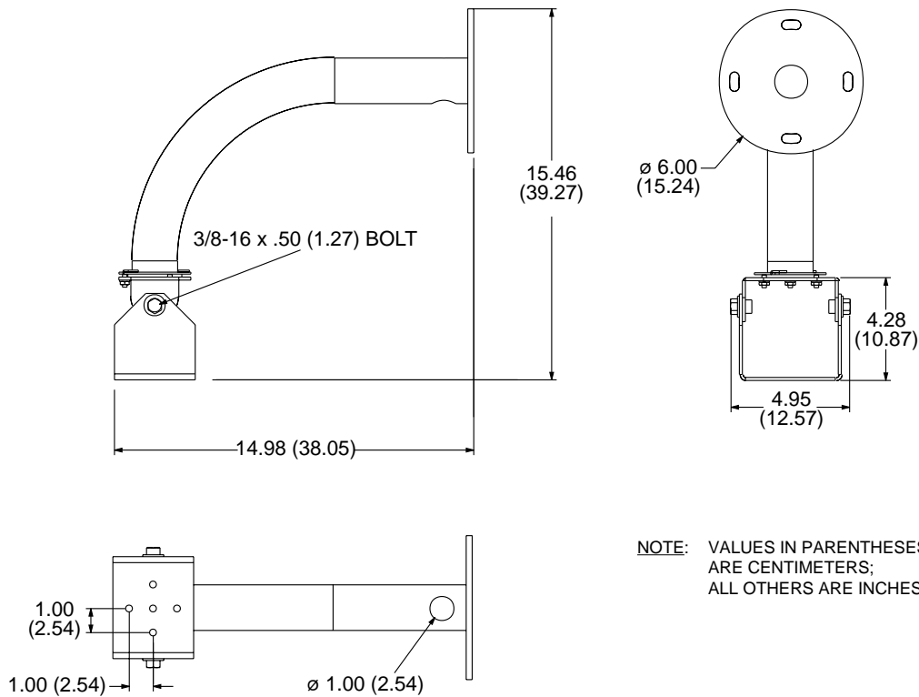
Figure 2. EM1900U Dimension Drawing
