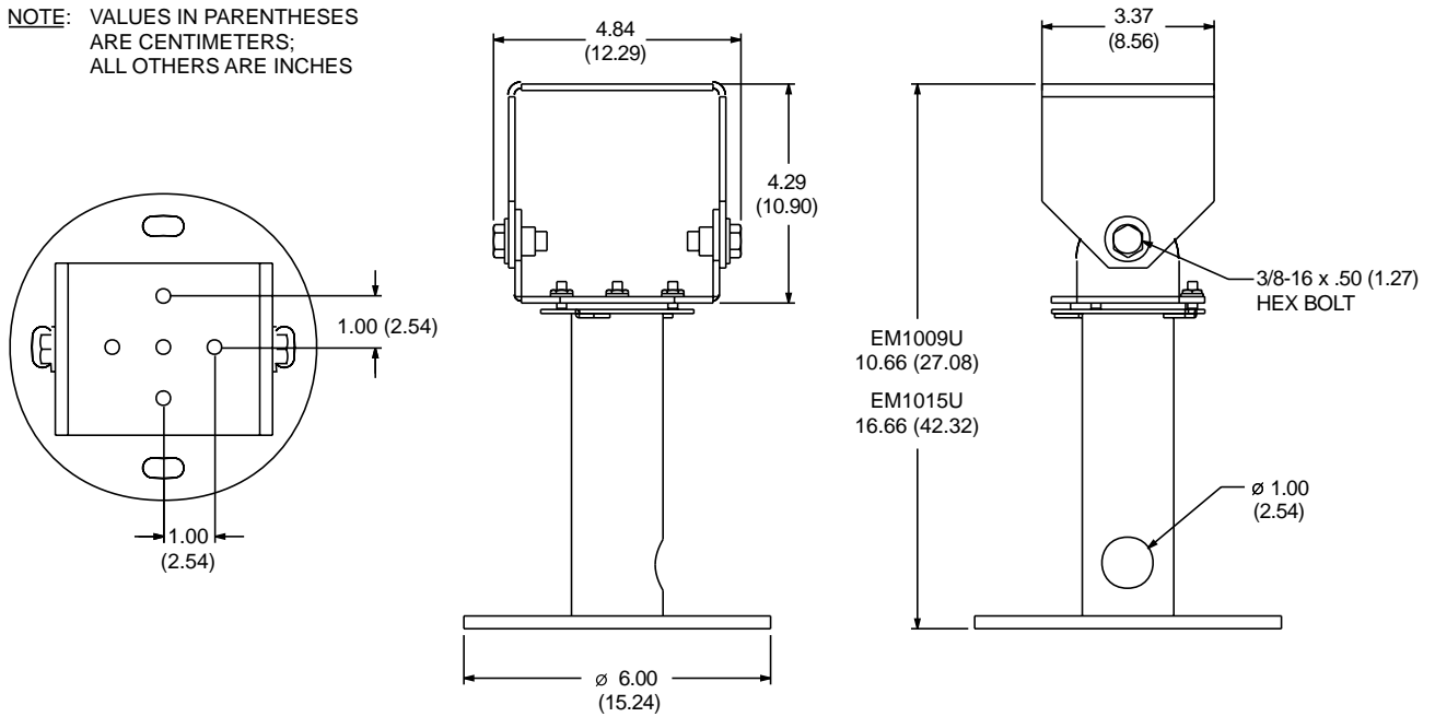
Figure 1. EM1009U/EM1015U Dimension Drawing
