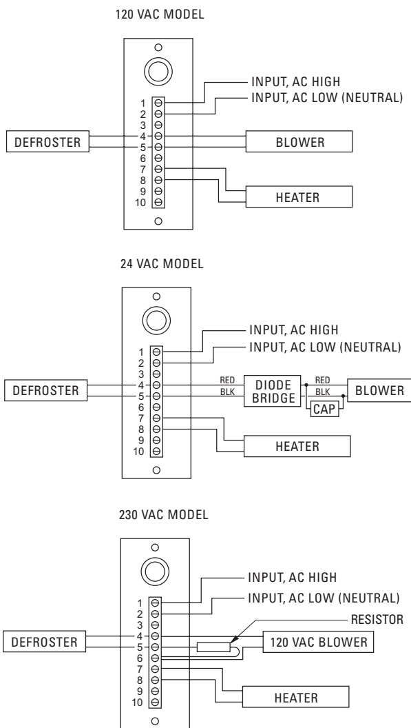
Figure 5. EH3512 Series Wiring Diagram
