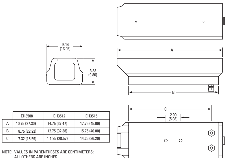
Figure 7. EH3508, EH3512, EH3515 Dimension Drawing
