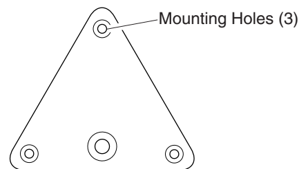
Three Mounting Holes for Solar Panel Base
