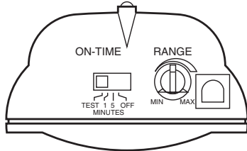
Bottom of Sensor
