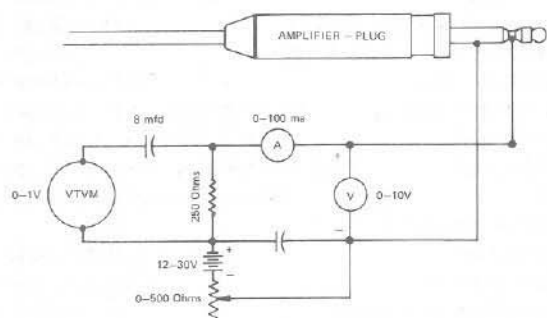
FIGURE 2 — Test Circuit
