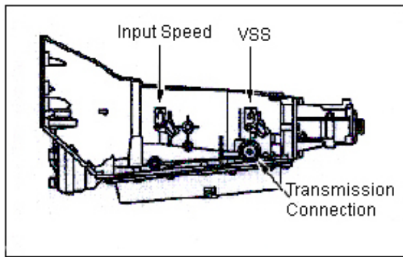
FIGURE 6.19 A/T Input Speed & VSS Sensor, Transmission Connection (4L80E)
