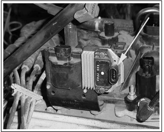
FIGURE 6.12 Coil Driver (Component is pictured on a 5.7. This image is used to show connector plug in, not component location)
