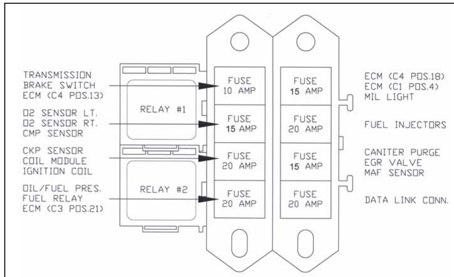
FIGURE 6.20 Fuse Identification
