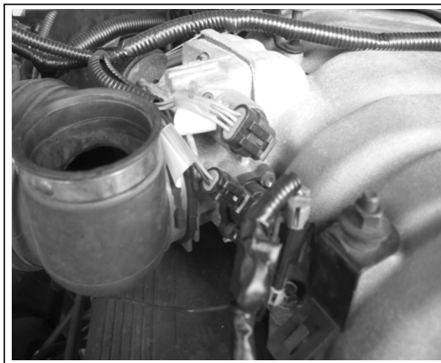
FIGURE 6.13 TPS Sensor and IAC Valve
