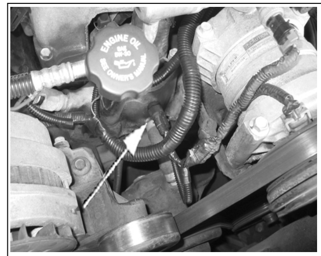
FIGURE 6.16 ECT Sensor
