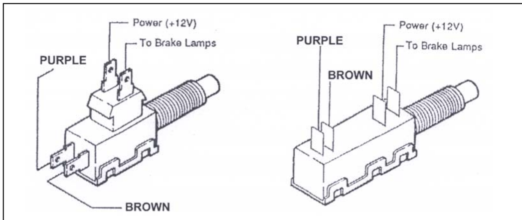
FIGURE 6.2 Brake Switch Connection
