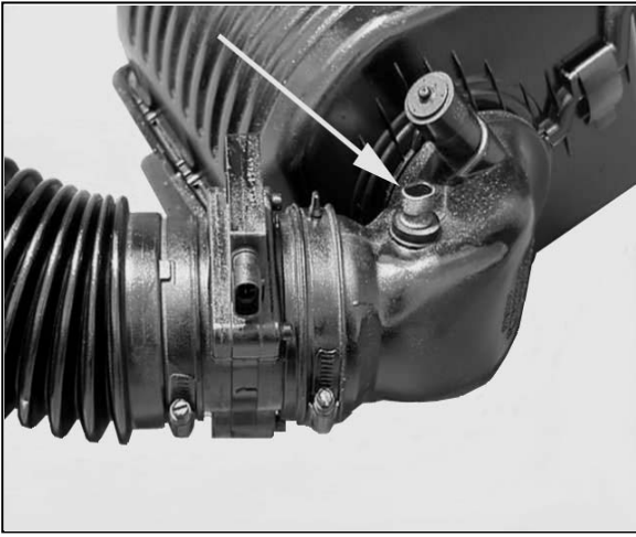
FIGURE 6.17 IAT Sensor
