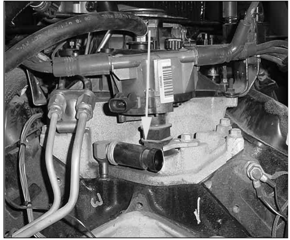
FIGURE 6.18 Fuel Pump/Oil PressureSwitch
