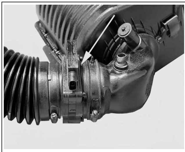
FIGURE 6.15 MAF Sensor
