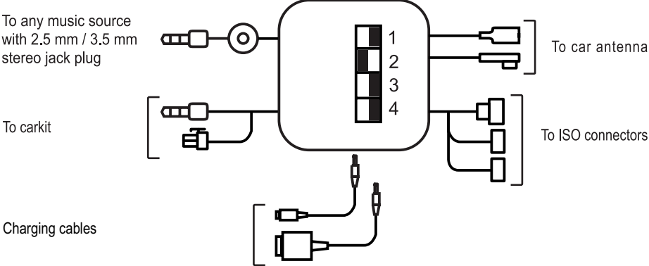
Illustration 4: installation scheme
