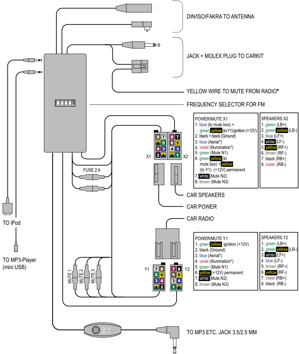
Illustration 4: installation scheme
