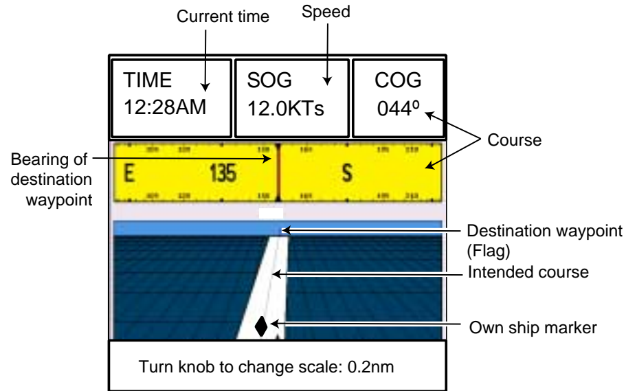
Highway display
