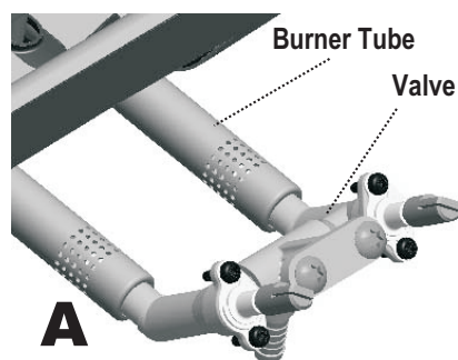
A Correct burner-to-valve engagement
