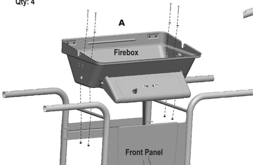
#10-24x1-1/4" Machine Screw Qty: 4
