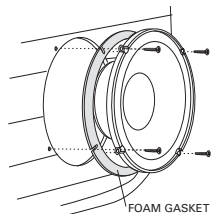
Figure 4. Mounting the 60.7cs woofer in a standard speaker location.
