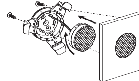
Figure 7D. In-dash location (may require gluing).
