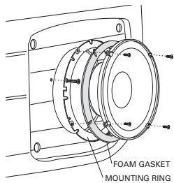
Figure 4. Mounting the 60.7cs woofer in a standard speaker location.
