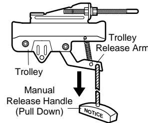
Manual disconnect position
