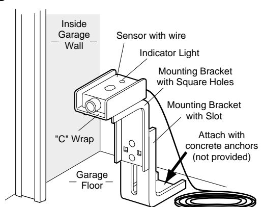
Figure 5 Alternate Floor Mount
