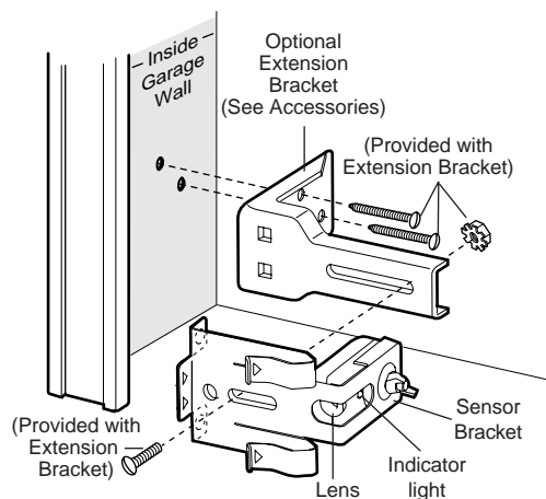
Figure 2 WALL MOUNT (Right Side)
