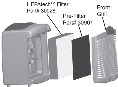
Figure 3 - Air Purifier Parts
