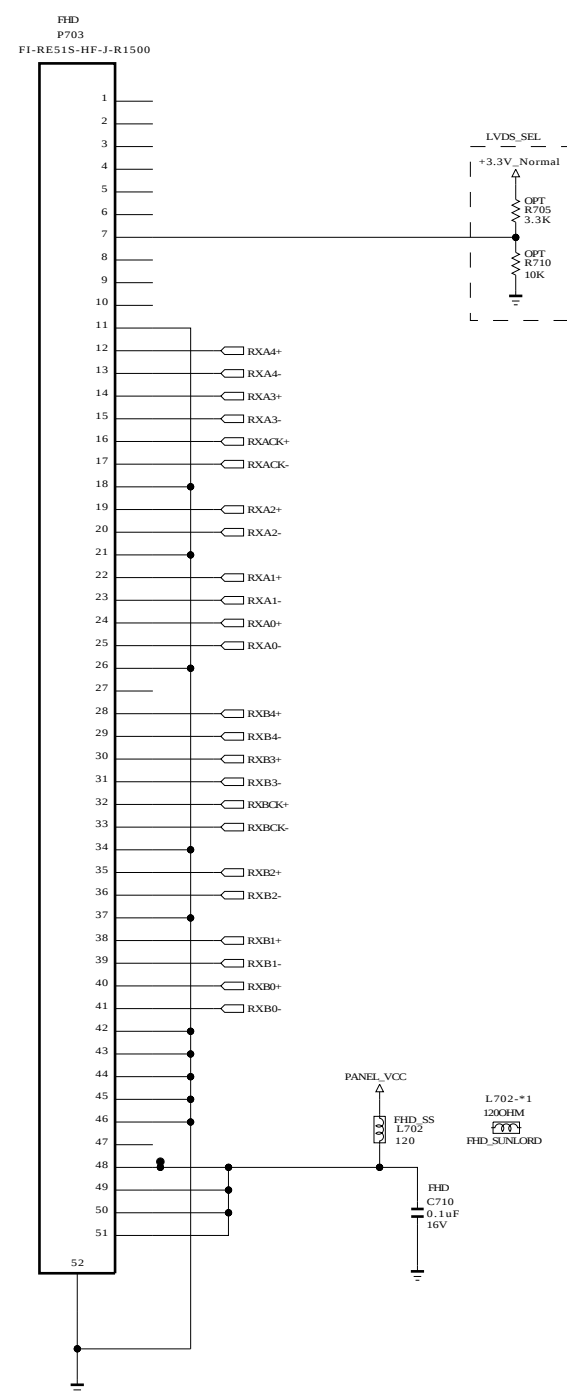
[51Pin LVDS Connector] (For FHD 60Hz)
