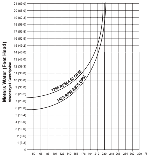
P316 NPSHR Chart
