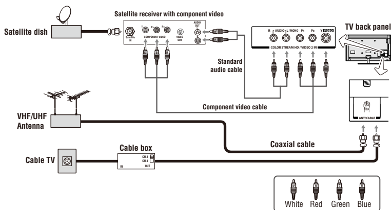
(Sample Illustration) L9300U Series—Connecting to an antenna, satellite receiver, and/or cable TV box
