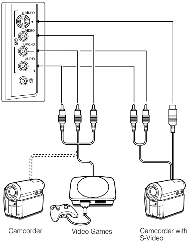
TV right side view
