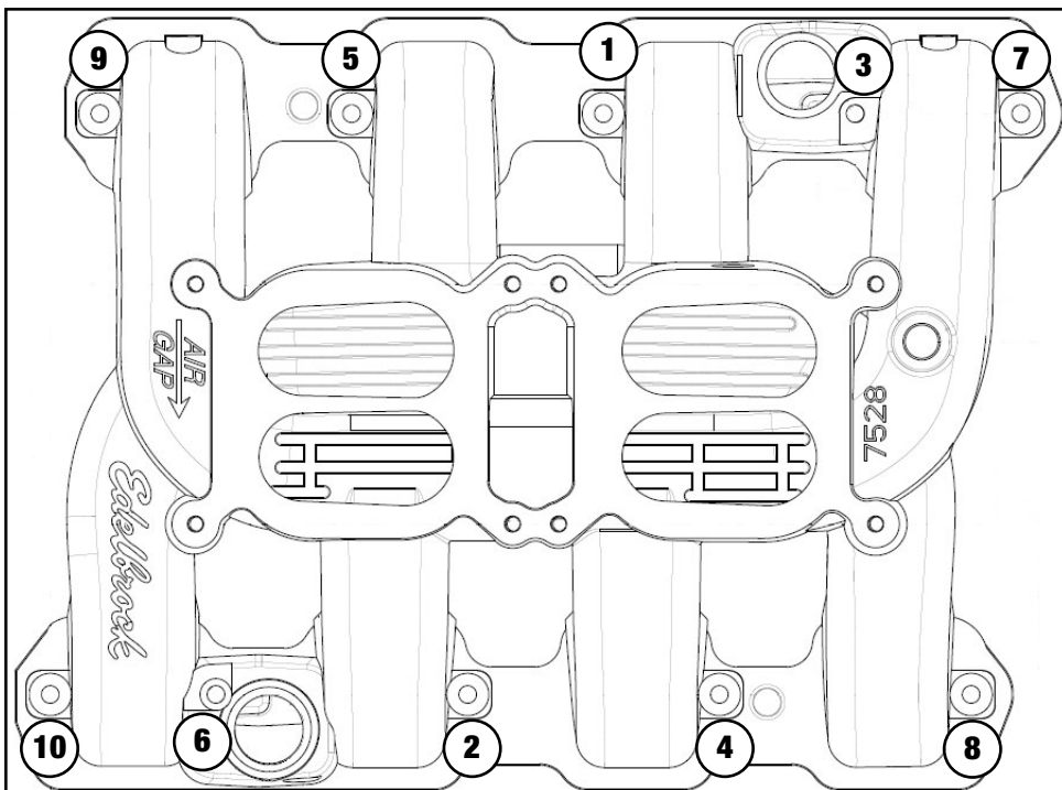
FIGURE 1 - Chrysler HEMI Dual Quad RPM Intake Manifold Torque Sequence
