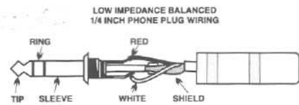
FIGURE 2 WIRING DIAGRAM
