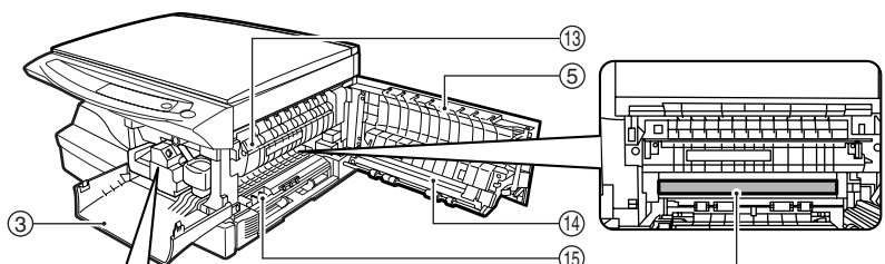
Photoconductive drum
