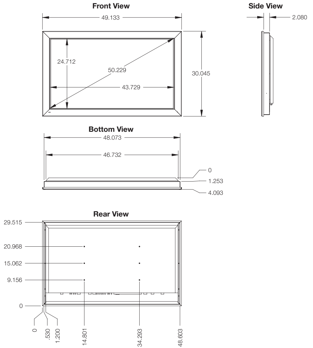
Figure 7-2. PlasmaWall Model PL-50DHD Dimensions
