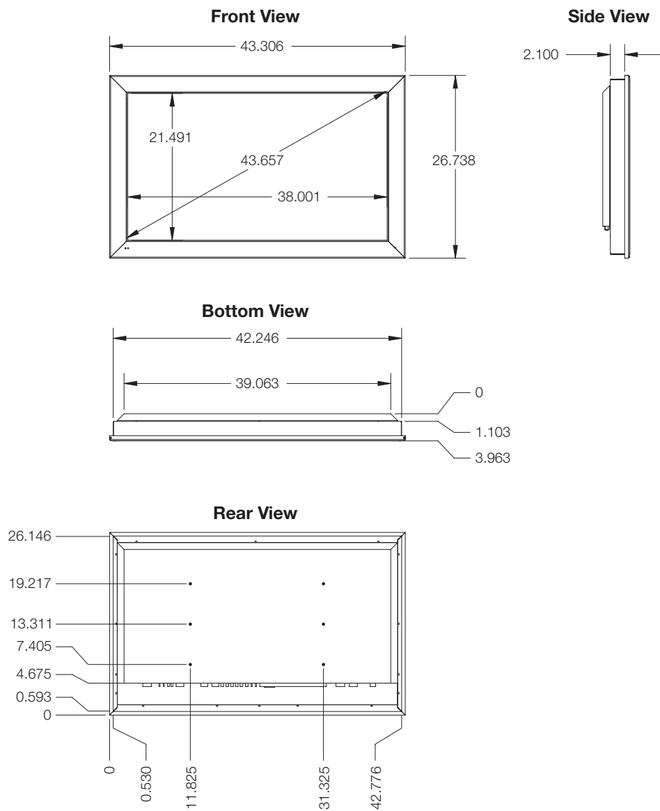
Figure 7-1. PlasmaWall Model PL-43DHD Dimensions
