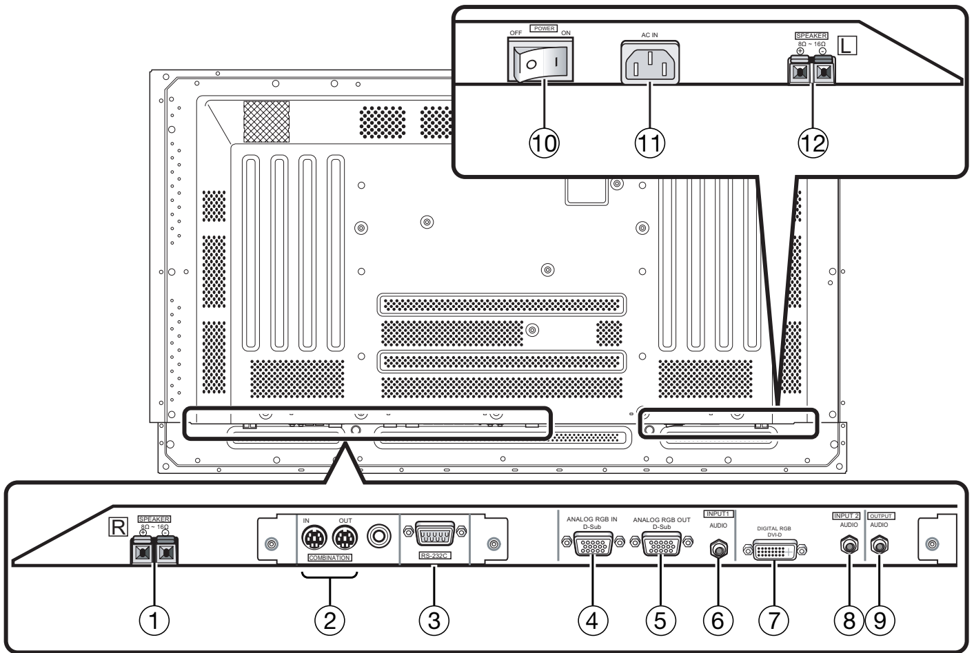
Figure 2-2. PlasmaWall Connectors
