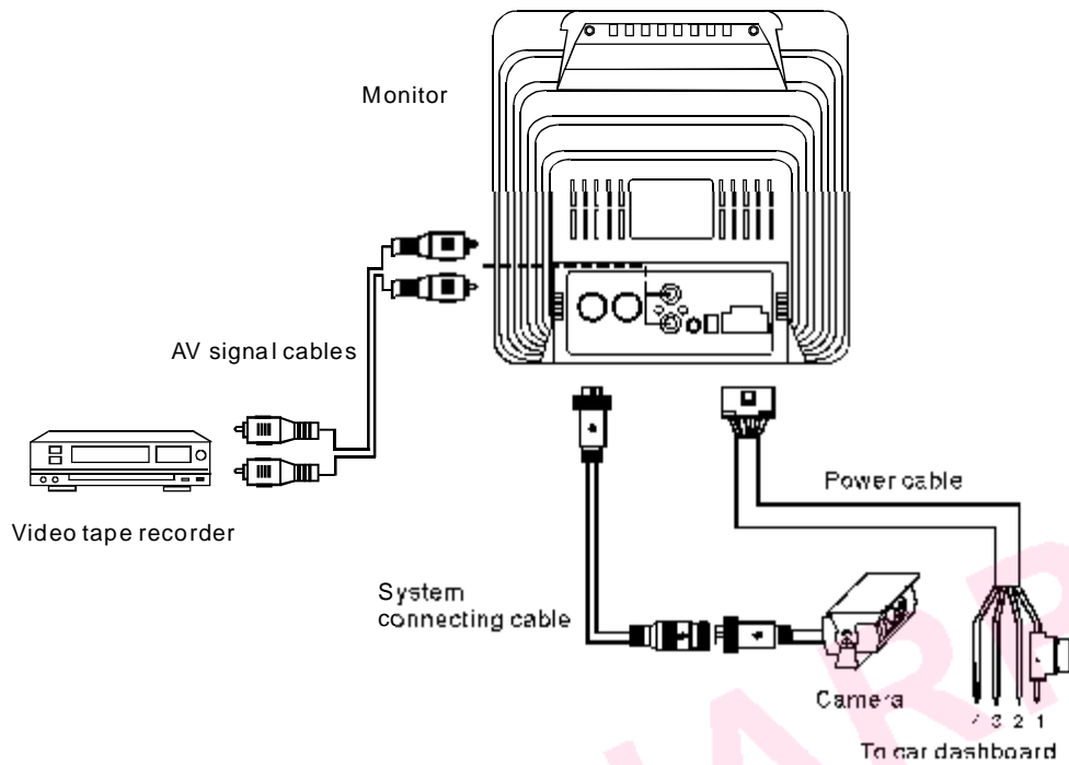
Fig 4 System connection
