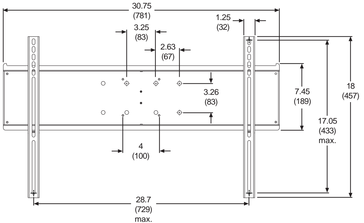
ADAPTER BRACKET DETAIL
