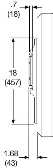
SIDE VIEW WITH DEEP BRACKET
