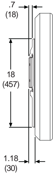
SIDE VIEW WITH SHALLOW BRACKET
