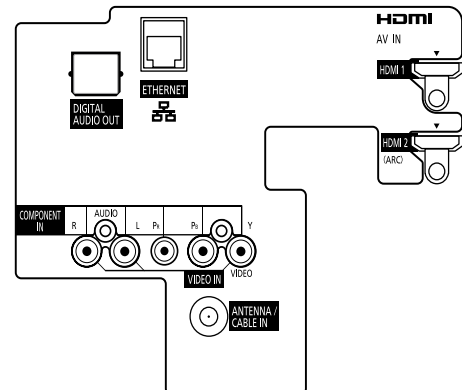
Rear Panel
