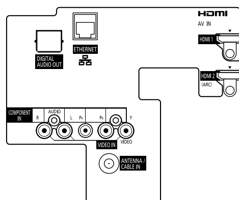
Rear Panel
