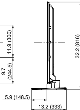
Side view with the pedestal (option) attached
