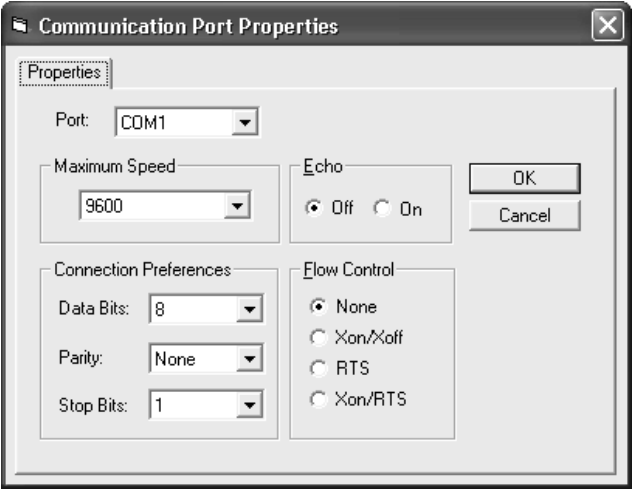
Communications Setup Menu Sets up the communications link between the FTG Configuration Application and the Z7 card installed in a TV/STB.
