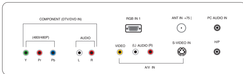
TV Rear
