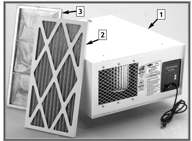
Figure 2. Model W1690 Deluxe Ceiling Mounted Air Cleaner and filters.
