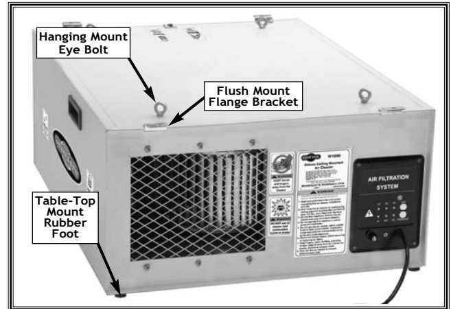
Figure 4. Air cleaner unit mounting options.
