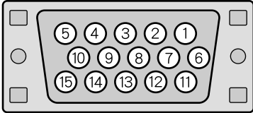
RGB input terminal (RGB INPUT/mD-sub)
