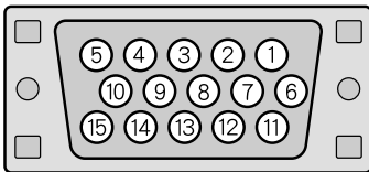
RGB2 input terminal (RGB2 INPUT/md-sub)
