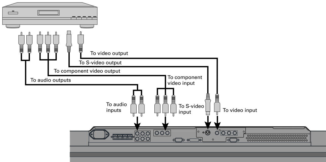
Bottom of Display (Ex.: P42VHA10)
