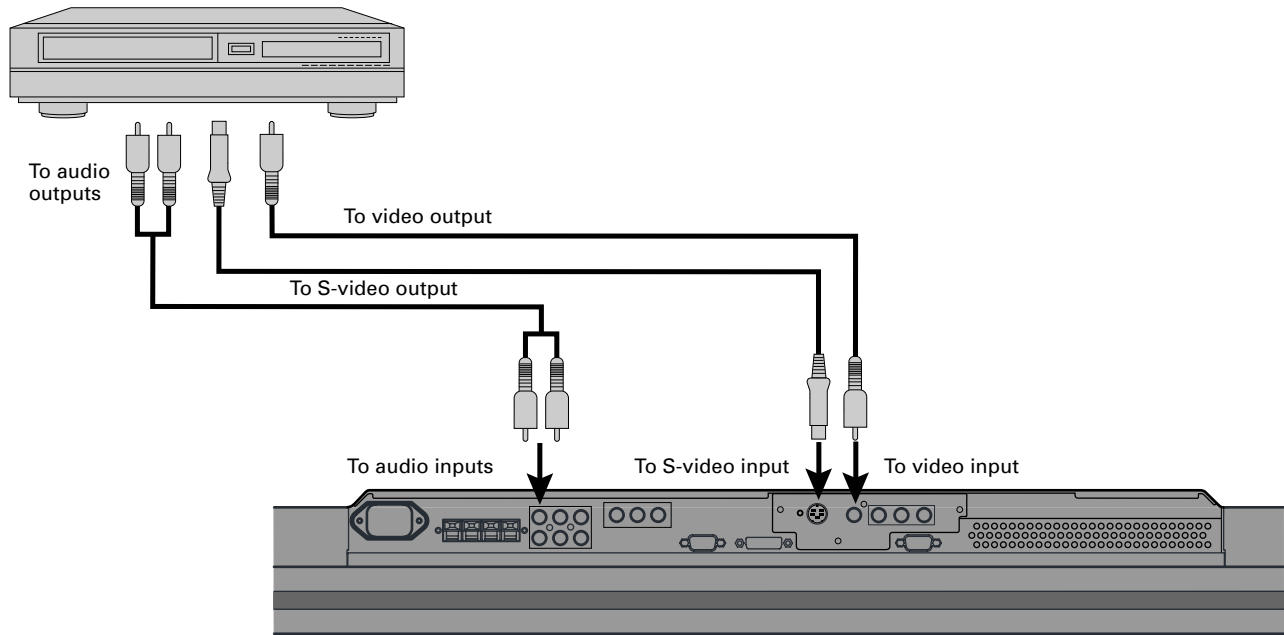
Bottom of Display (Ex.: P42VHA10)
