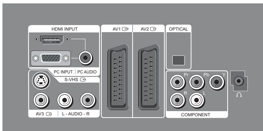
Rear Panel
