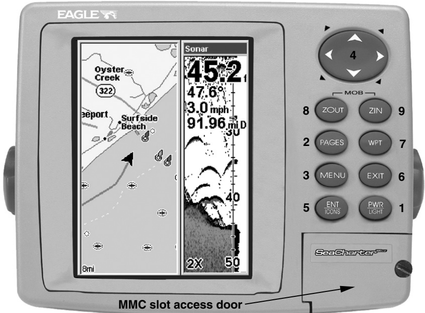
SeaCharter 500CDF sonar/GPS unit, front view, showing map with sonar chart screen display, keyboard and access door for the MMC slot.
