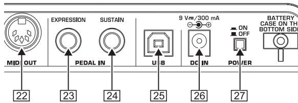
Fig. 3.3: Rear panel connectors
